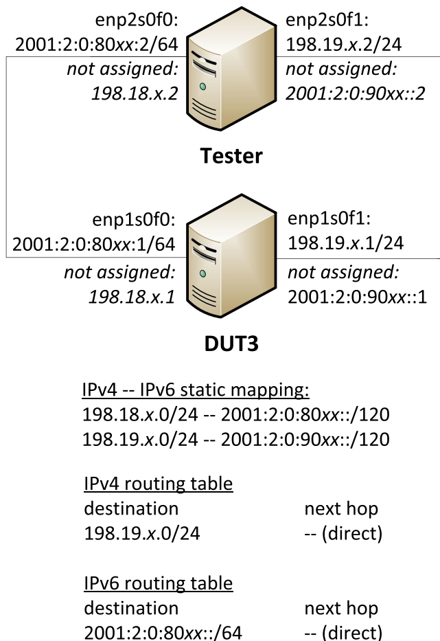
FIGURE 10 Single DUT test setup for benchmarking SIIT gateways, DUT3 implements stateless NAT64.
